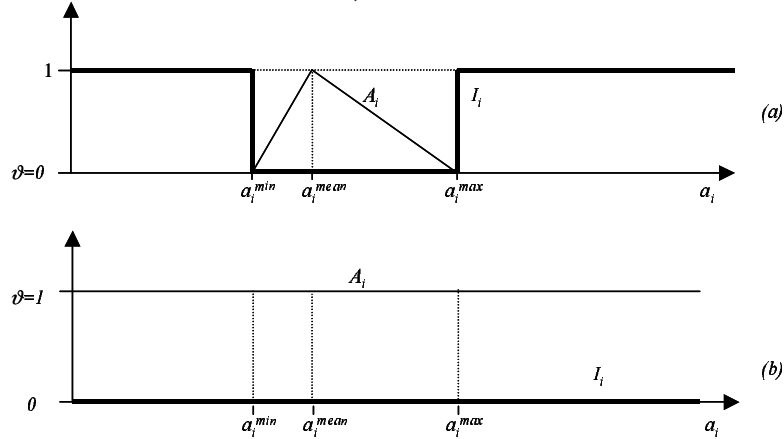
Fig. 4. Fuzzy sets A_i and I_i when (a) \vartheta=0 and (b) \vartheta=1 .
