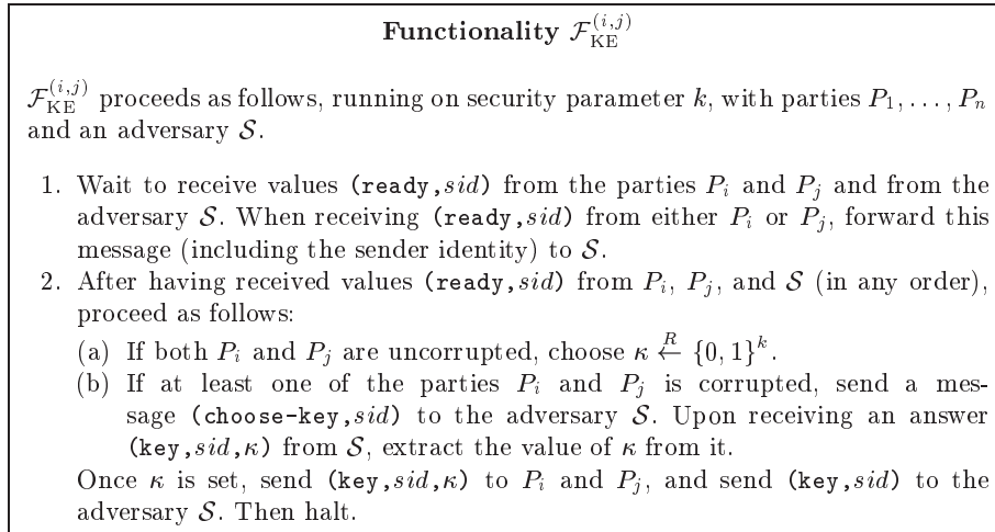
Fig. 1. The modified key exchange functionality \mathcal{F}_{\text{KE}}^{(i,j)}
