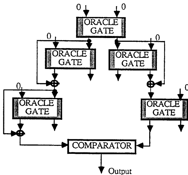
Figure 1. Deterministic distinguishing circuit for \psi(f, f, f^2)
